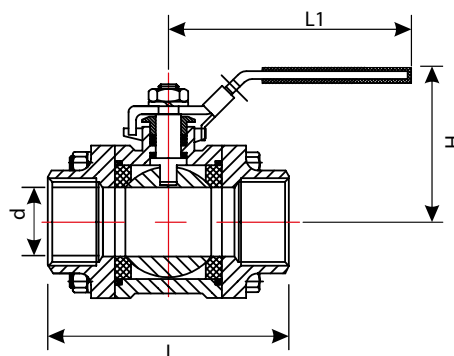
PN63 Threaded Ball Valve with Lever
